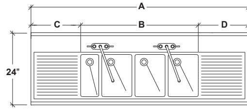
'D' SERIES PLAN VIEW
