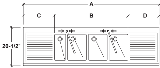
'S' SERIES PLAN VIEW
