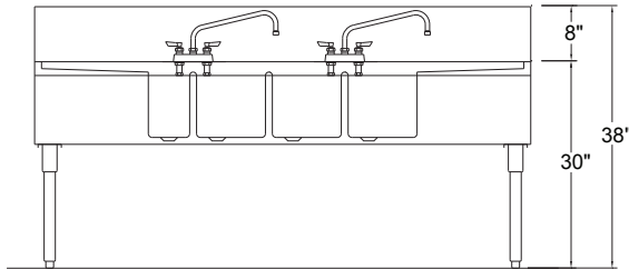
'S' SERIES ELEVATION
