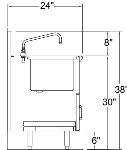
'D' SERIES SECTION (WITH OPTIONAL CABINET BASE)
