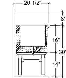
'S' SERIES SECTION
