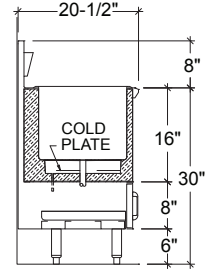
'S' SERIES SECTION
