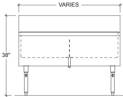
TYPICAL SECTION
