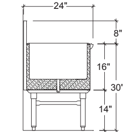
'D' SERIES SECTION
