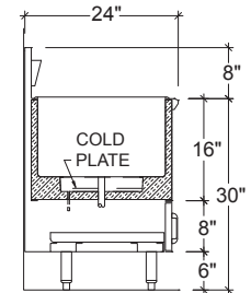
'D' SERIES SECTION
