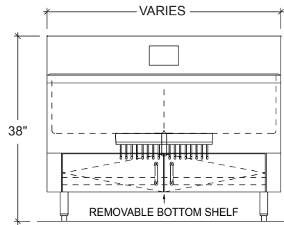
TYPICAL ELEVATION (WITH OPTIONAL COLD PLATE AND CABINET BASE)
