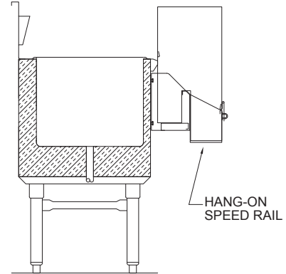
LOCKING COVER SECTION VIEW
