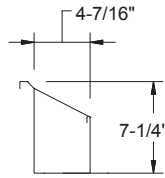
SPEEDRAIL SECTION VIEW
