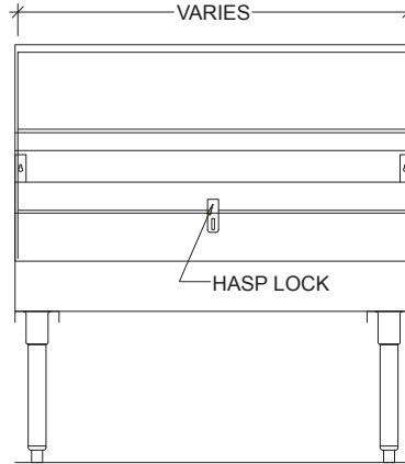
LOCKING COVER ELEVATION VIEW
