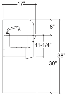
SECTION
