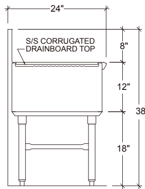
'D' SERIES SECTION
