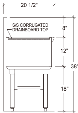
'S' SERIES SECTION
