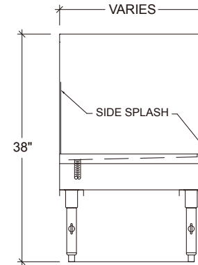
'S' or 'D' SERIES RECESSED ELEVATION
