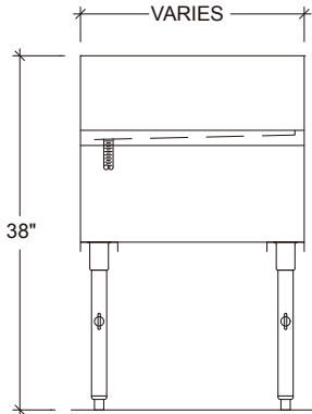
'S' SERIES ELEVATION
