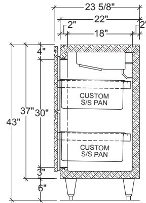
STANDARD SECTION
