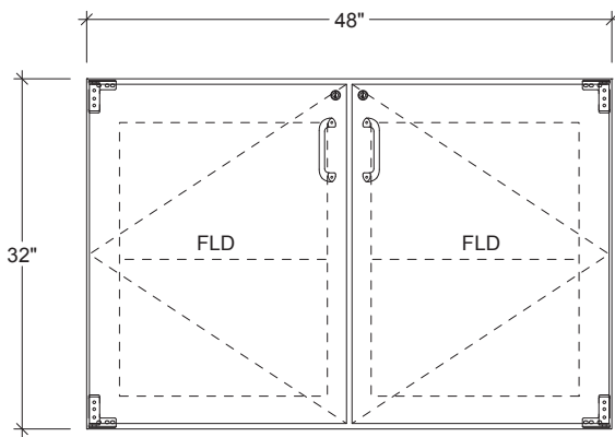
TYPICAL ELEVATION
