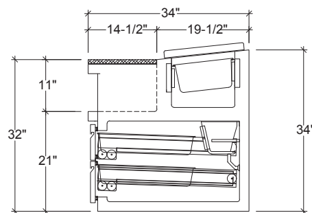
DRAWER SECTION
