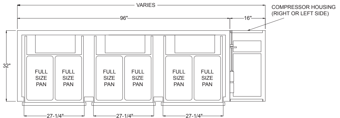
PLAN VIEW MODEL SHOWN: IRSL-3-06
