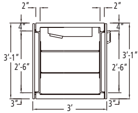
SECTION 36" BODY
